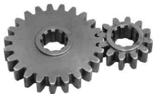
Spur Gear 12x23 Inner 10S Part No. NR 1051
