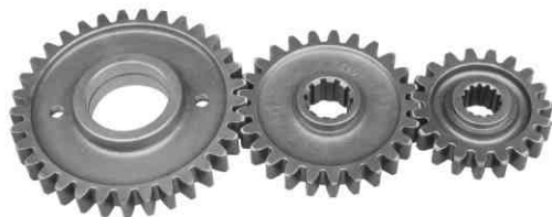
Side Gear Set 33T x 25T x 19T (Inner 14S) Part No. NR 879
